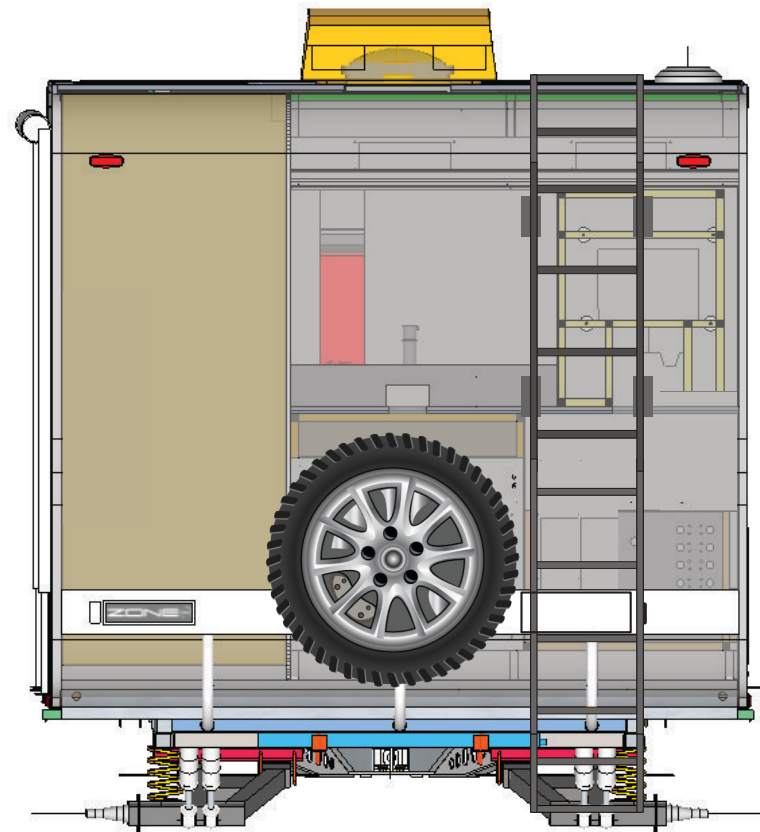
Operating Position
