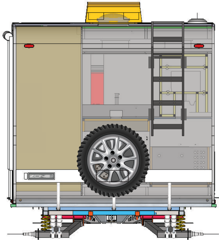
Travelling Position
